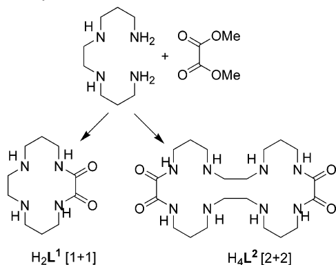
Scheme 1. Synthesis of H_2L^1 [1 + 1] and H_4L^2 [2 + 2] Macrocyclus a
